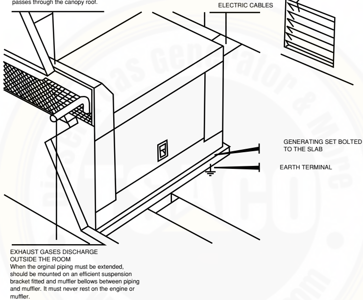
Figure 3.7. Soundproof type Generating set room
